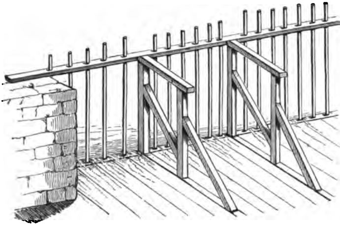
Fig. 254.—Wooden grating to serve as a boom.
